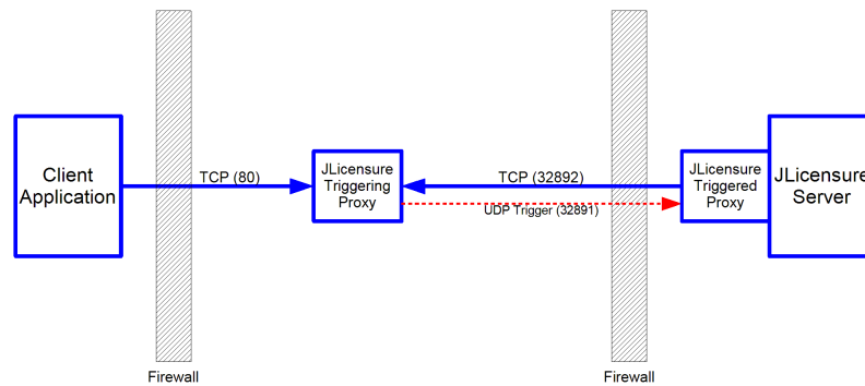
Figure 4: Secure Server
